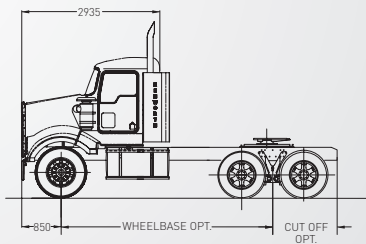
T409SAR DAY CAB
