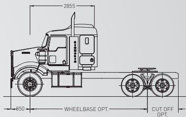
T409SAR 36" SLEEPER RECESSED BACK
