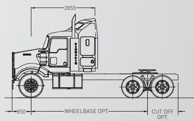
T409SAR 36" SLEEPER RECESSED BACK
